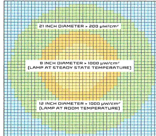
BEAM PROFILE AT 15 INCHES
