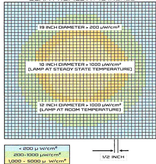
BEAM PROFILE AT 12 INCHES
